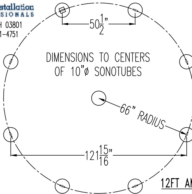
SONOTUBE LAYOUT
